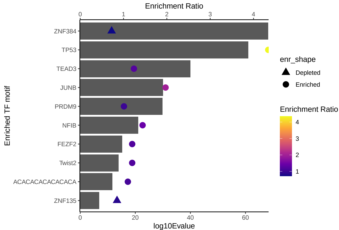
H3K27ac_Set3_data - 10
